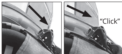
5) Align the visor over each retainer, matching the notch with the button and push until you hear a click.
